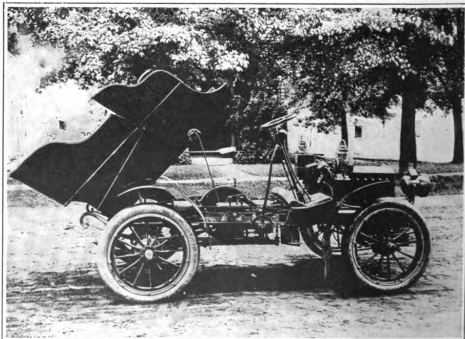
SHOWING BODY OF "MODEL" CAR RAISED FOR INSPECTION OF MACHINERY.
